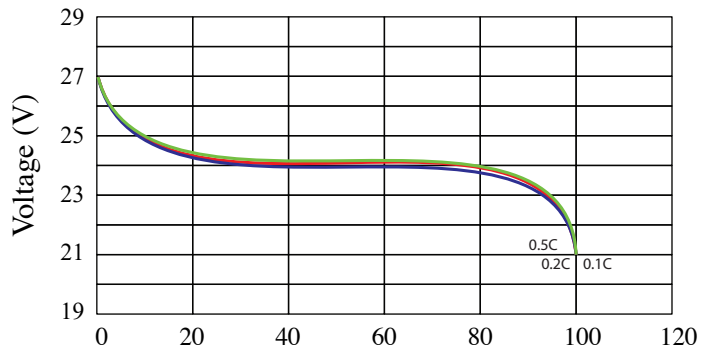
Discharge Performance at 40°C
