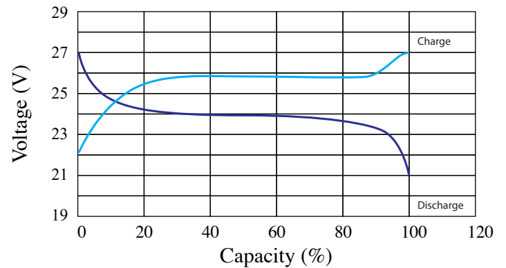
Charge and Discharge at 40°C, 0.5C
