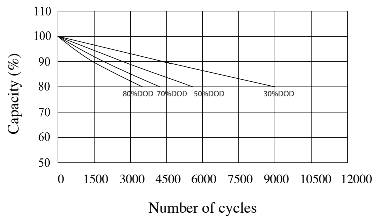
Cycle Life with DOD at 35°C, 0.3C
